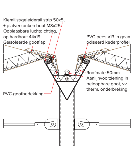
GOOTDETAIL
